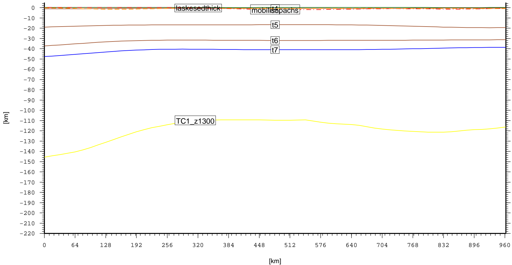
Cross section – SIB.TurgaySyncline (topo, laske sedthick, t4, t5, t6, t7)
