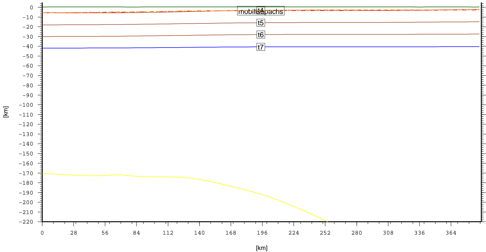
Cross section – SIB.KatangaSaddle (topo, laske sedthick, t4, t5, t6, t7)
