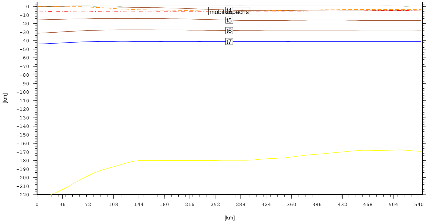
Cross section – SIB.BaykitAnteclise (topo, laske sedthick, t4, t5, t6, t7)
