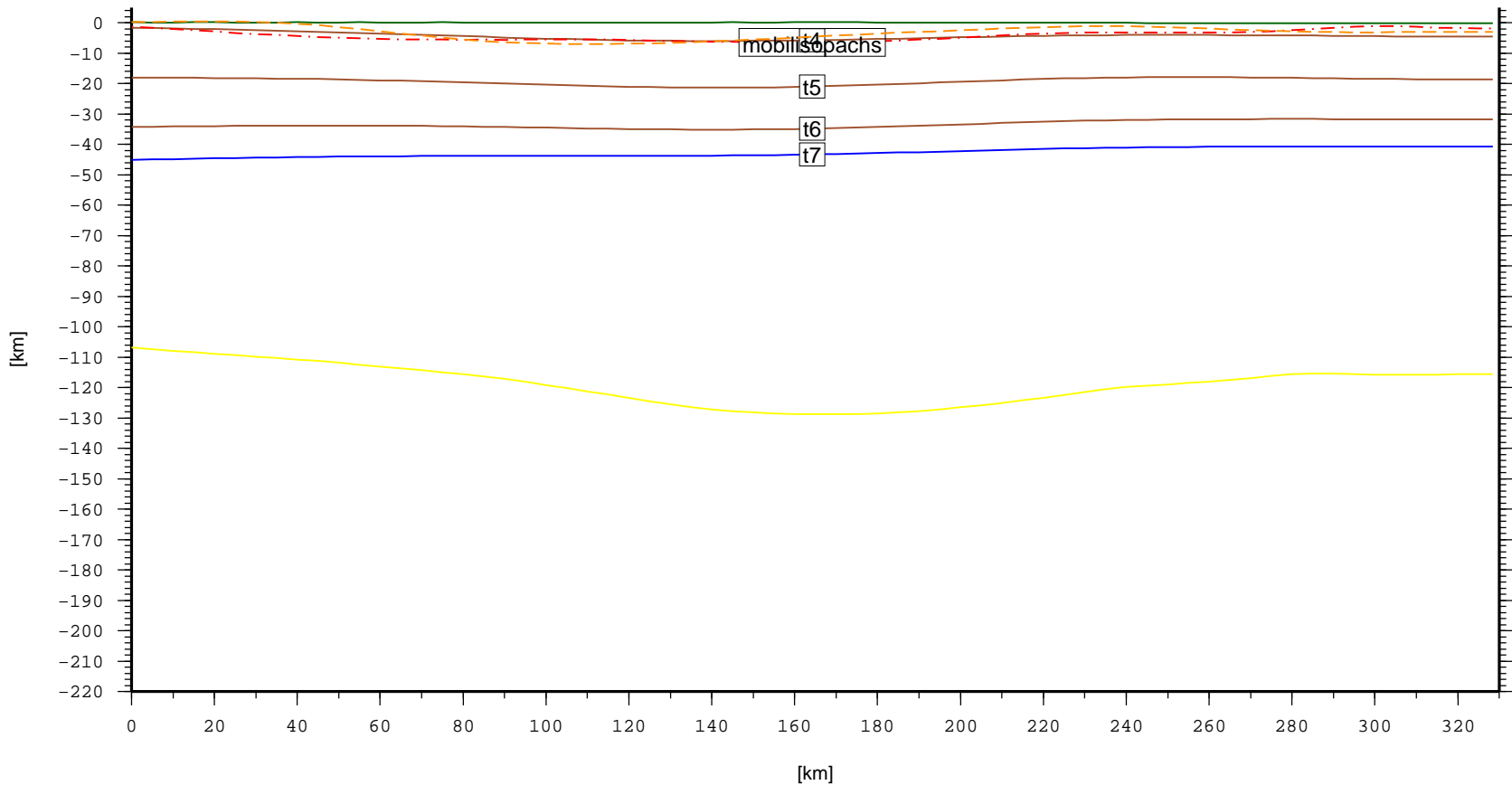
Cross section – SIB.BaydaratskayaTrough (topo, laske sedthick, t4, t5, t6, t7)
