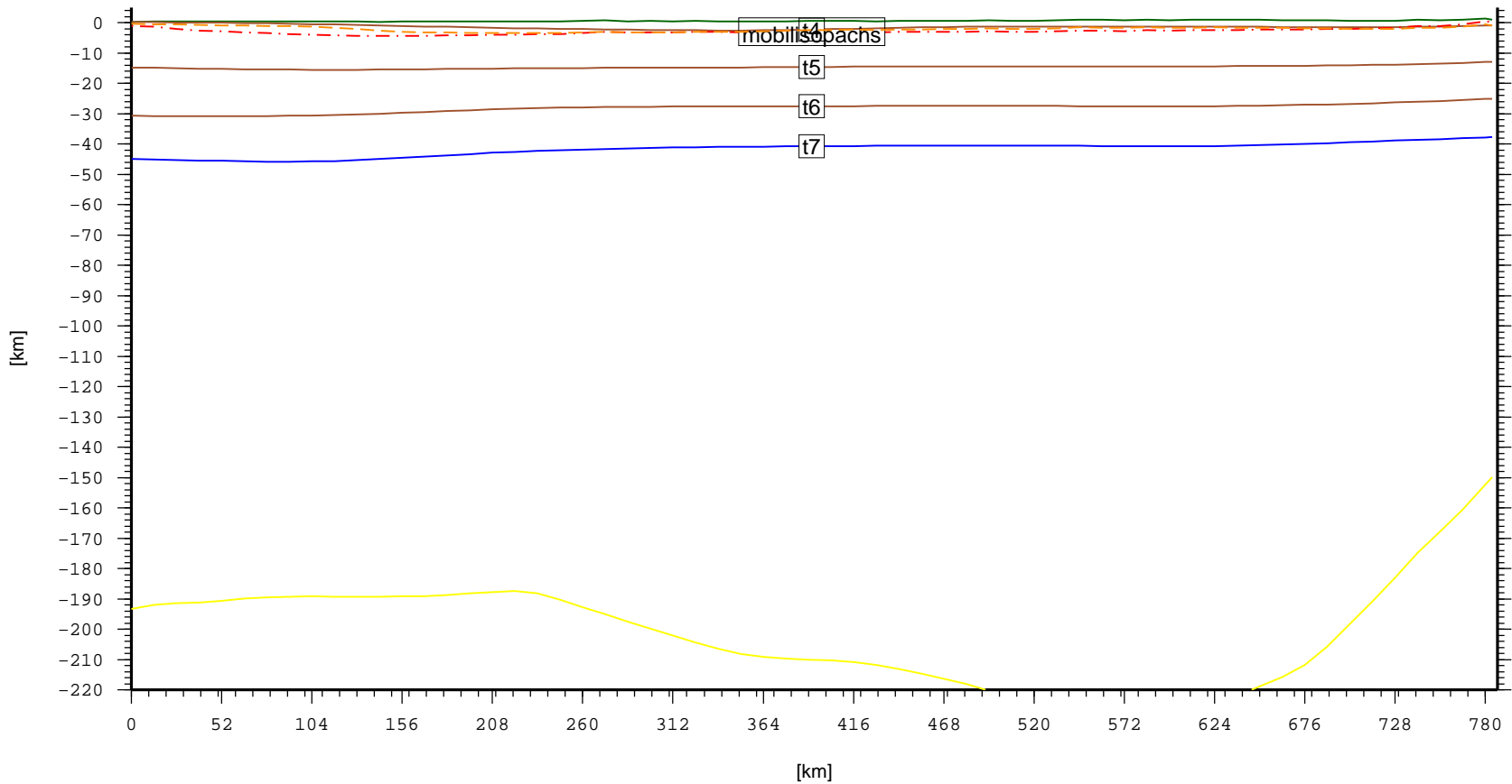
Cross section – SIB.Angara–LenaStructuralTerrace (topo, laske sedthick, t4, t5, t6, t7)
