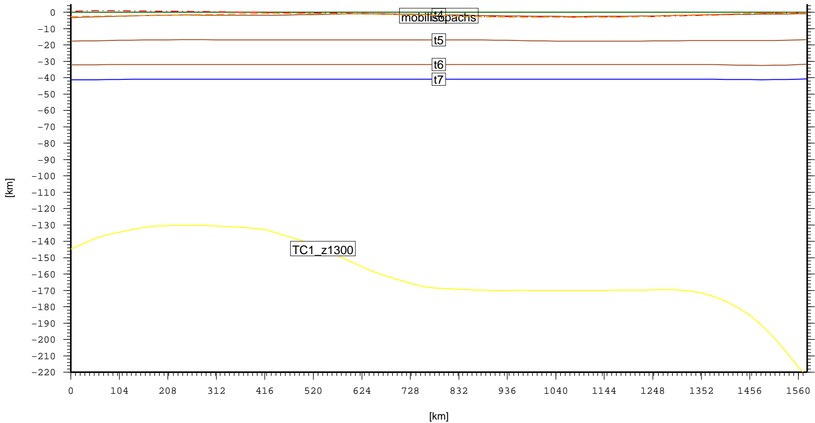
Cross section – SAM.Solimoes_UpperAmazonBasin (topo, laske sedthick, t4, t5, t6, t7)
