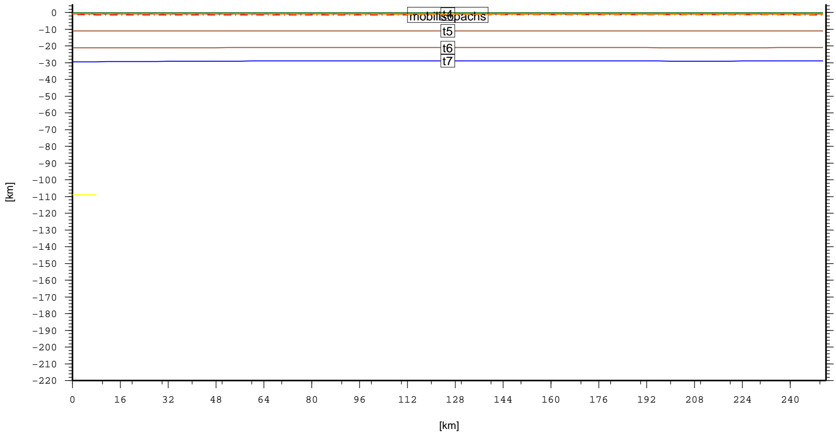
Cross section – SAM.SanJulianBasin (topo, laske sedthick, t4, t5, t6, t7)
