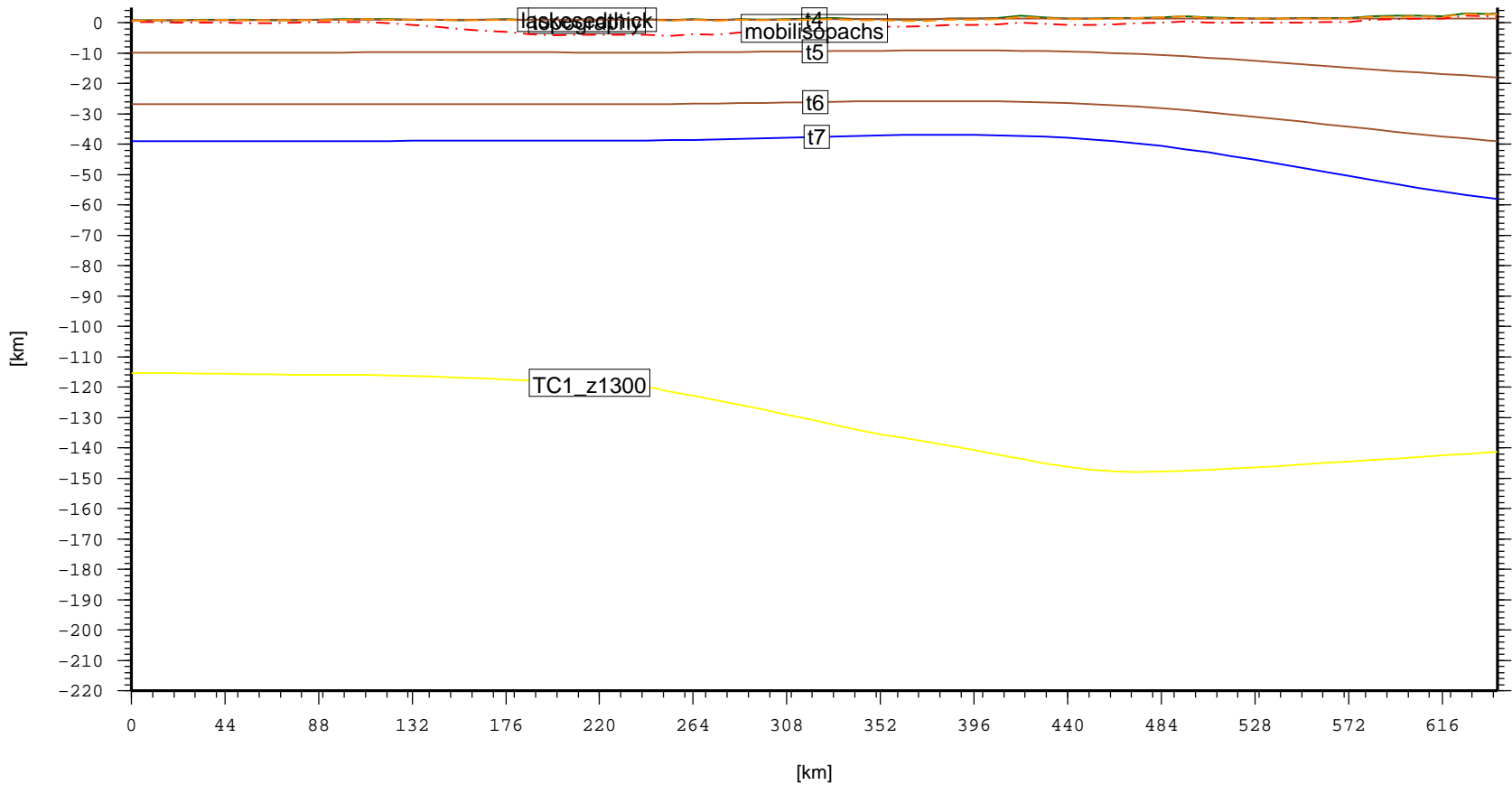
Cross section – SAM.NeuquenBasin (topo, laske sedthick, t4, t5, t6, t7)
