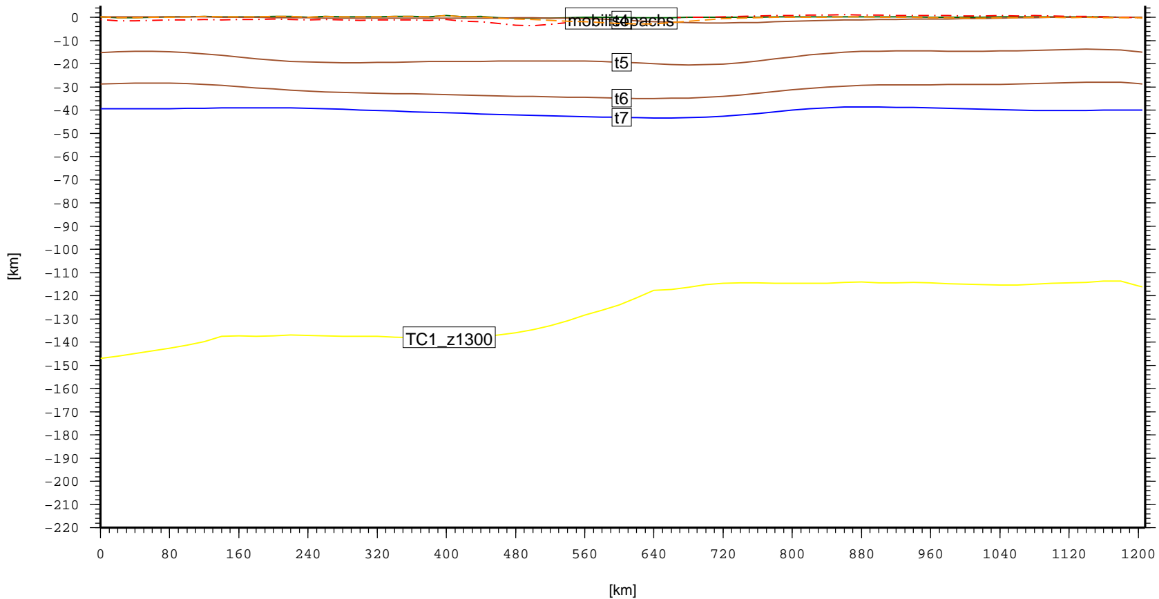
Cross section – NAM.AnticostiBasin (topo, laske sedthick, t4, t5, t6, t7)
