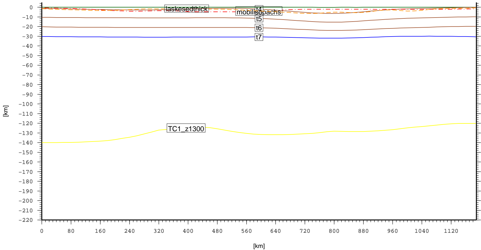
Cross section – CHN.BohaiGulfBasin (topo, laske sedthick, t4, t5, t6, t7)
