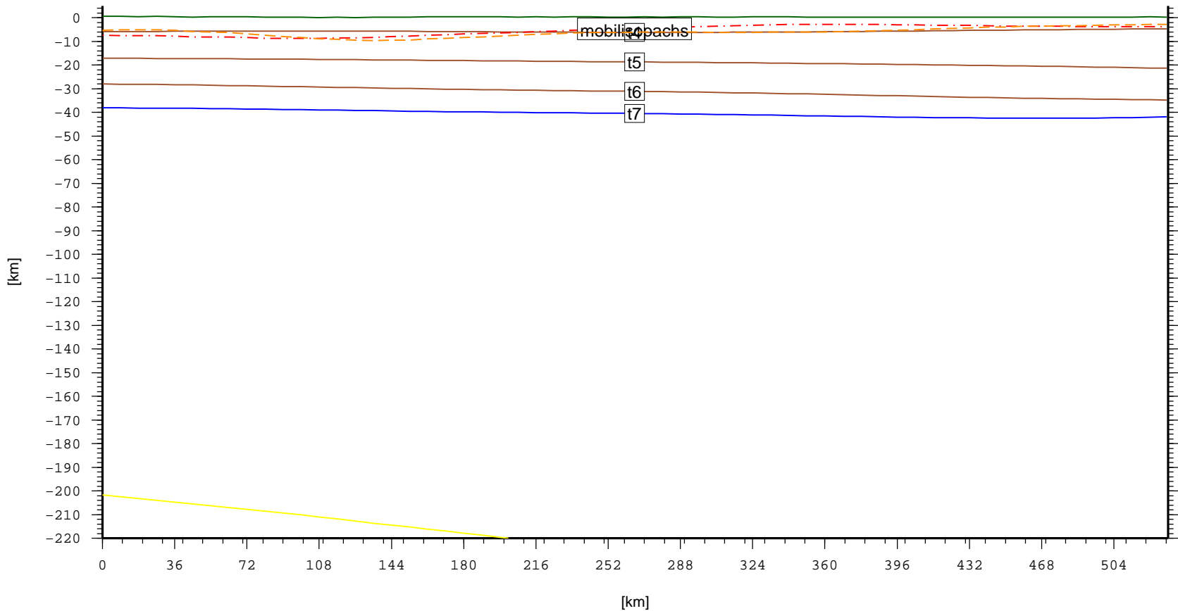
Cross section – CAS.Kama–KinelGrabenSystem (topo, laske sedthick, t4, t5, t6, t7)
