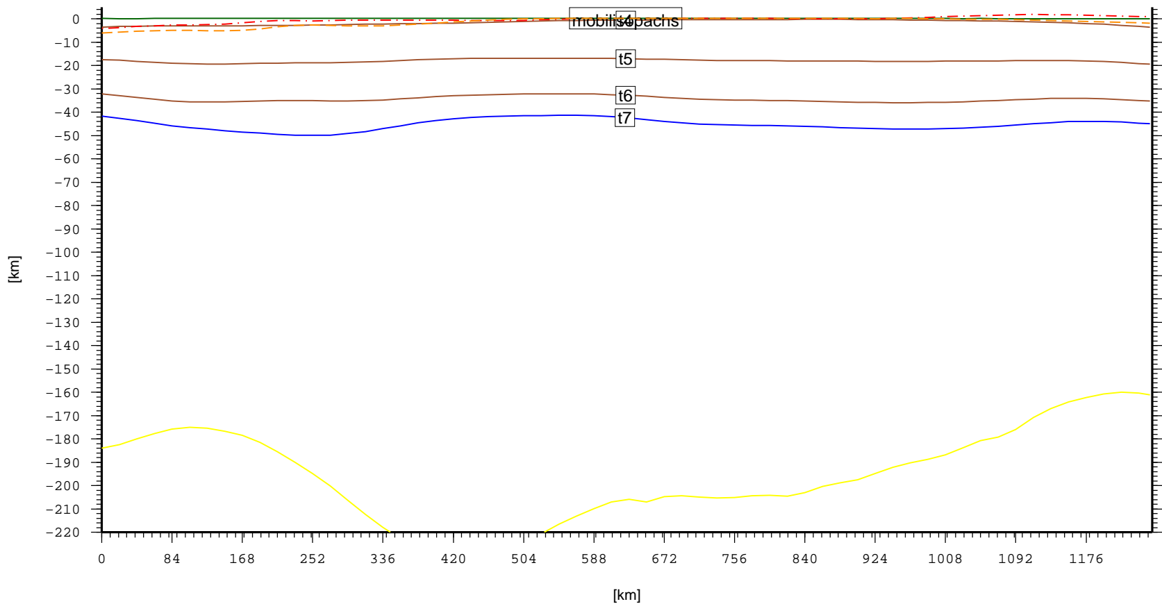
Cross section – CAS.EastEuropeanPlatform (topo, laske sedthick, t4, t5, t6, t7)
