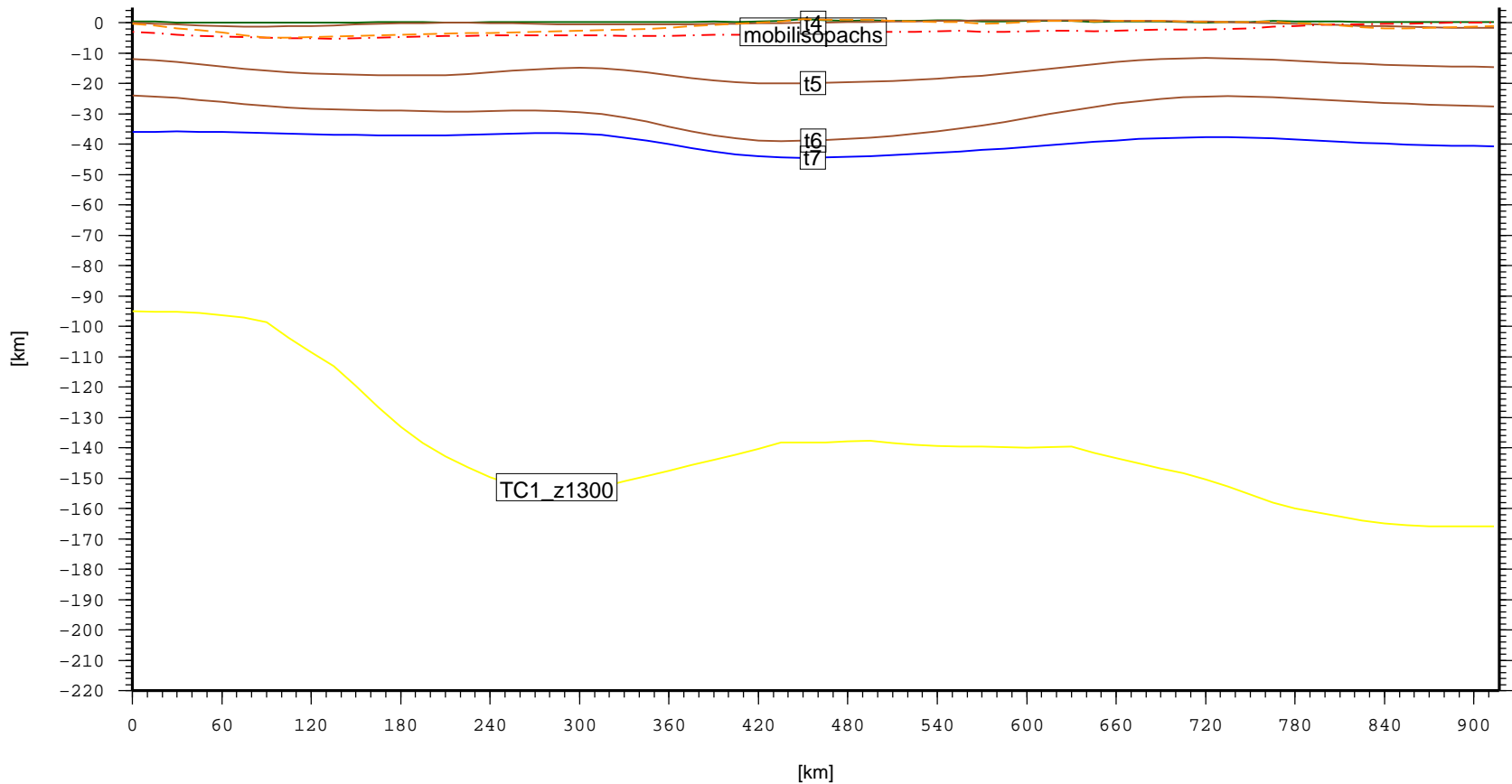
Cross section – ARC.NorthernInteriorPlatform (topo, laske sedthick, t4, t5, t6, t7)
