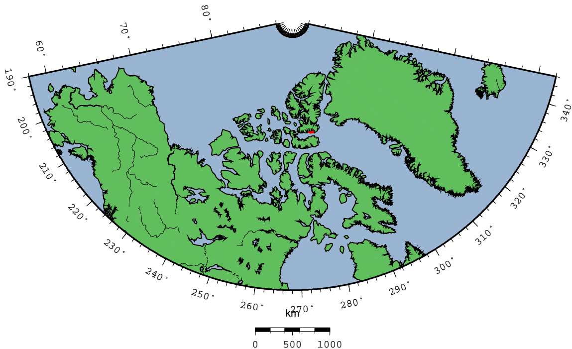
Location map ARC.NorthJonesBasin.
