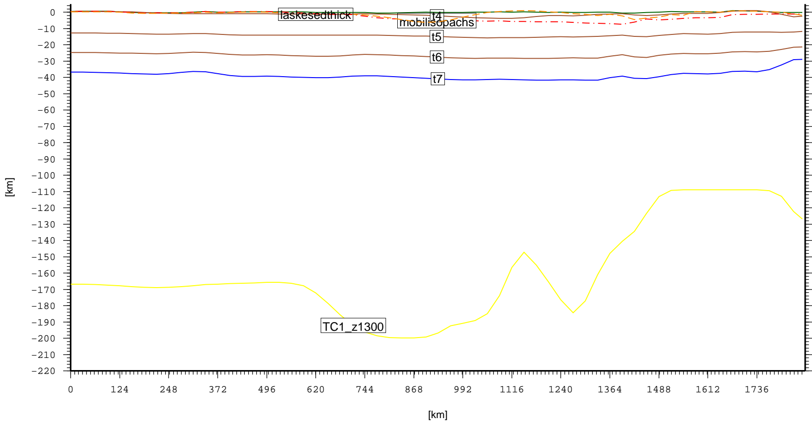
Cross section – ARC.ArcticStablePlatform (topo, laske sedthick, t4, t5, t6, t7)
