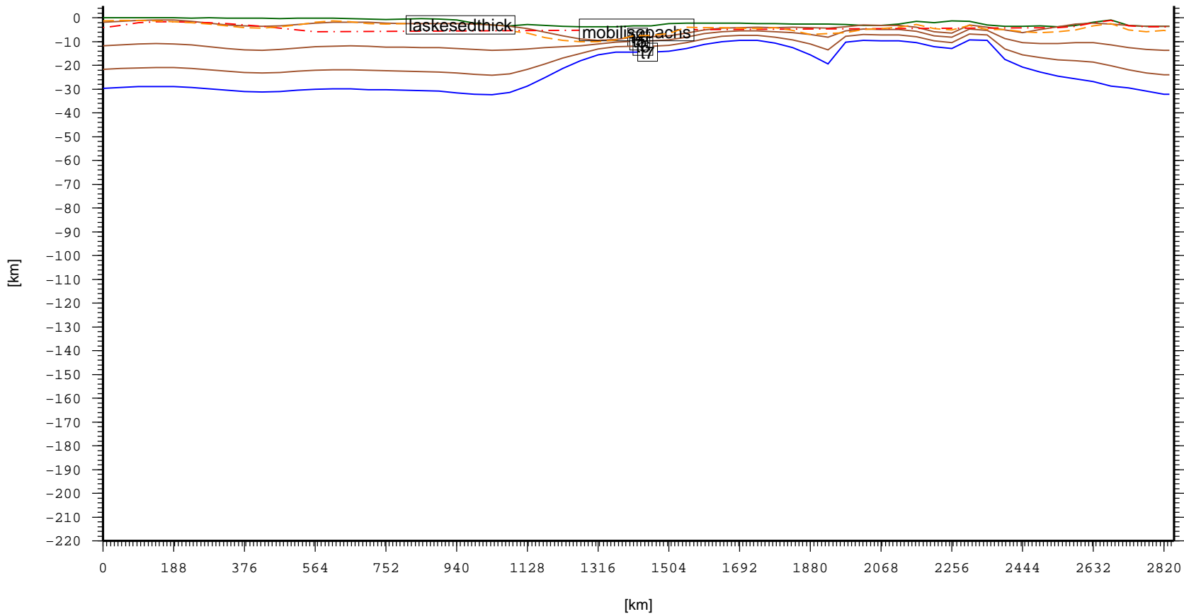
Cross section – ARC.ArcticCoastalPlain (topo, laske sedthick, t4, t5, t6, t7)
