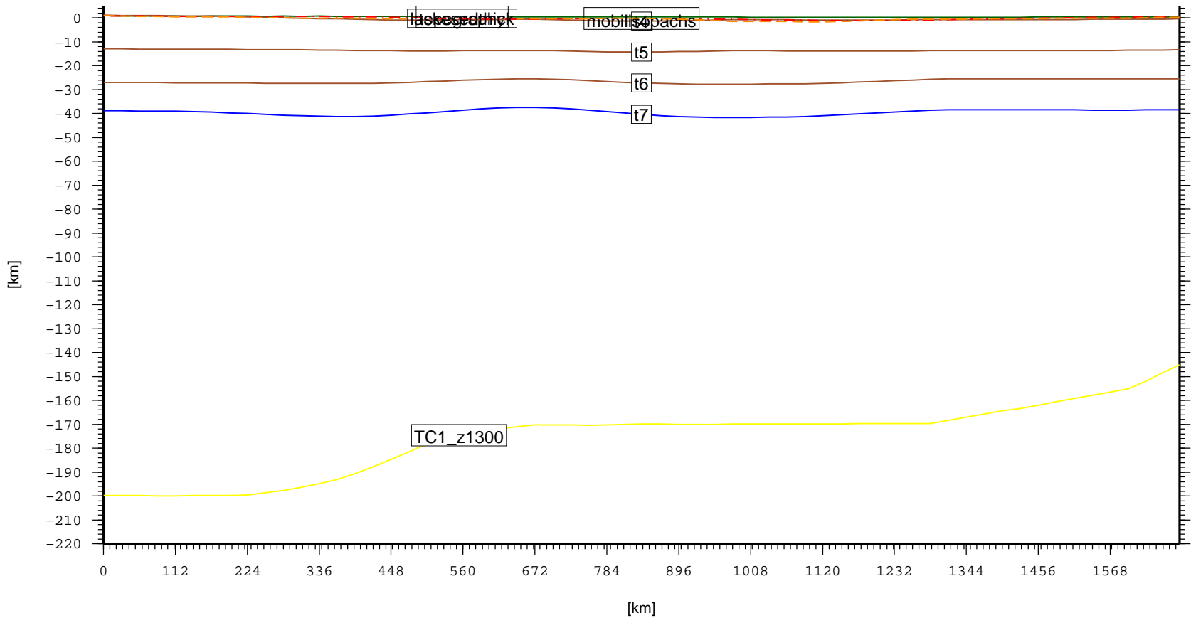
Cross section – AFR.ChadBasin (topo, laske sedthick, t4, t5, t6, t7)
